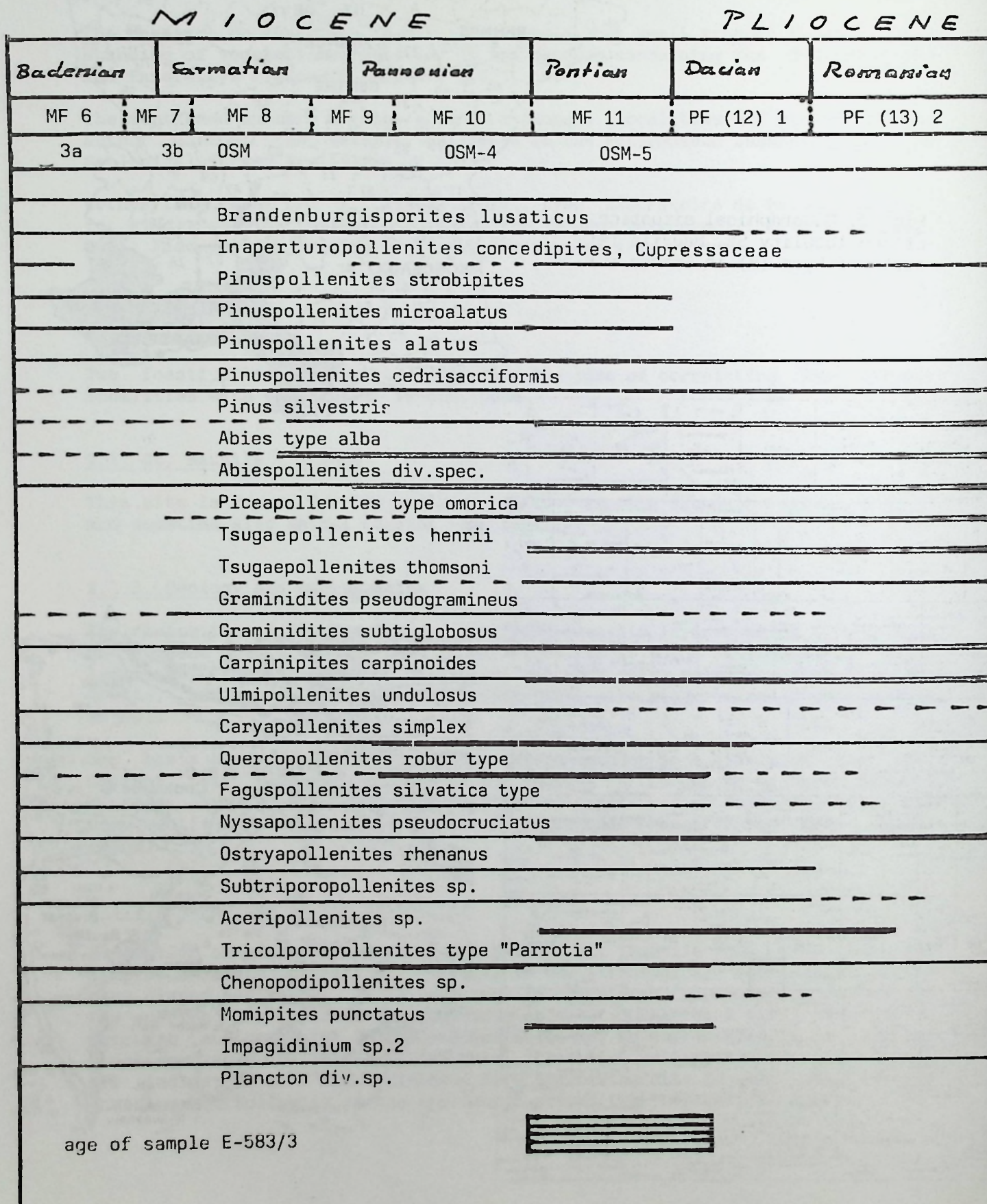
Fig. 2: Stratigraphical range of the mentioned sporomorphs from sample E 583/3 St. Bauzile
