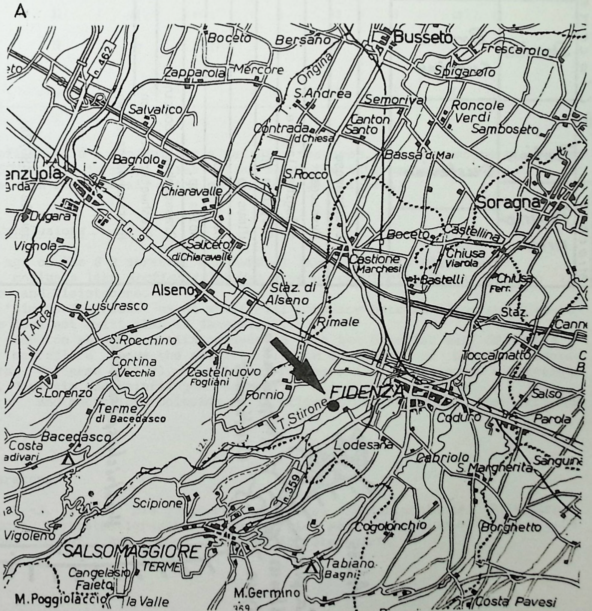
Fig. 3: Geographical situation of the Stirone profile near Fidenza (A) in Upper Italy (B).
