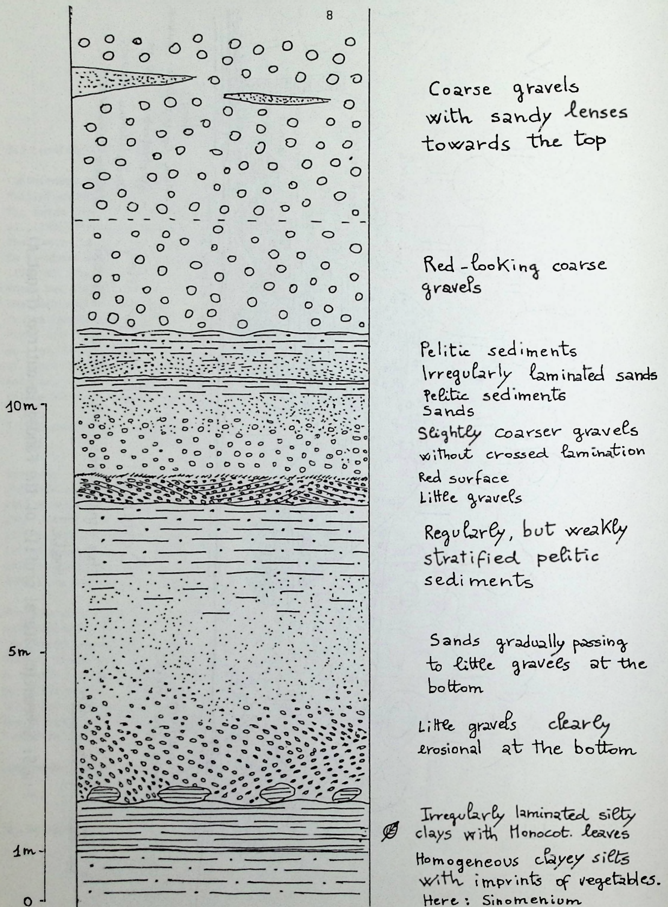
Fig.6: Part of the profile from Fig.5 at the place where the fossil Sinomenium came out (Front A).
